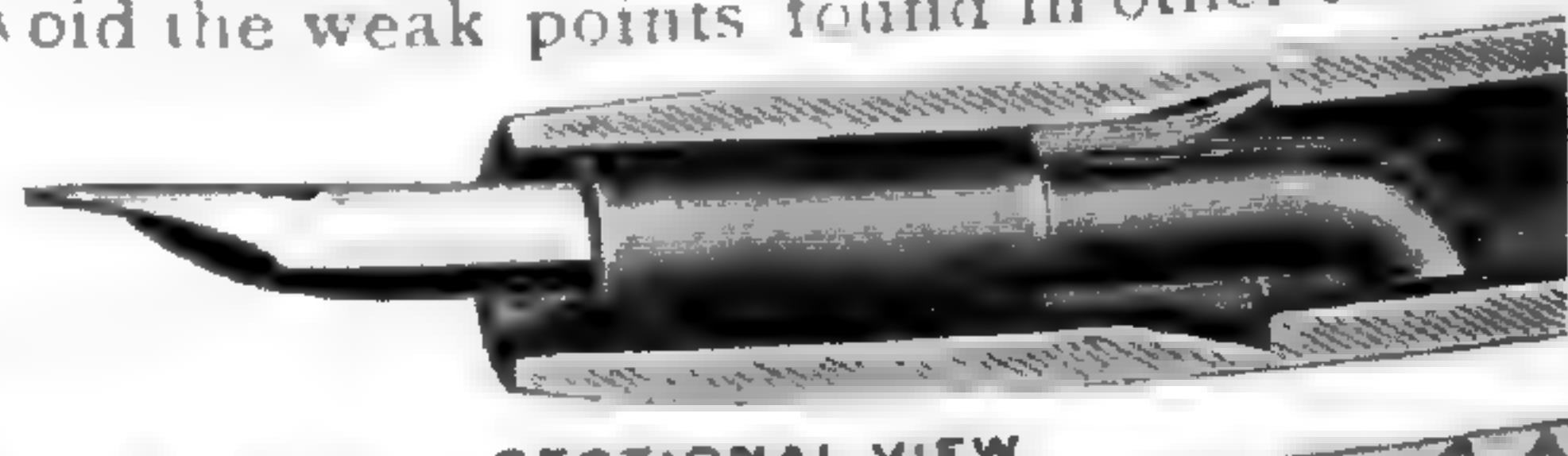
SECTIONAL VIEW.
